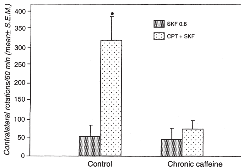
Figure 3. Influence of N 6 -cyclopentylthioephyllyline (CPT, 7.2 mg/kg) on the turning behaviour induced by SKF 38393 (0.6 mg/kg) in control and caffeine-treated 6-hydroxydopamine-lesioned rats. Left: ("control"): CPT (7.2 mg/kg, 15 min before) significantly potentiated SKF 38393-induced turning in control rats. Right: "chronic caffeine": rats received caffeine (1 g/l in their drinking water) over 14 days. At the end of chronic treatment, they were treated with SKF 38393 alone (0.6 mg/kg) or CPT (7.2 mg/kg) plus SKF 38393. Each group was composed of six animals. * p < .005 versus SKF 38393 alone according to Student's t test.
